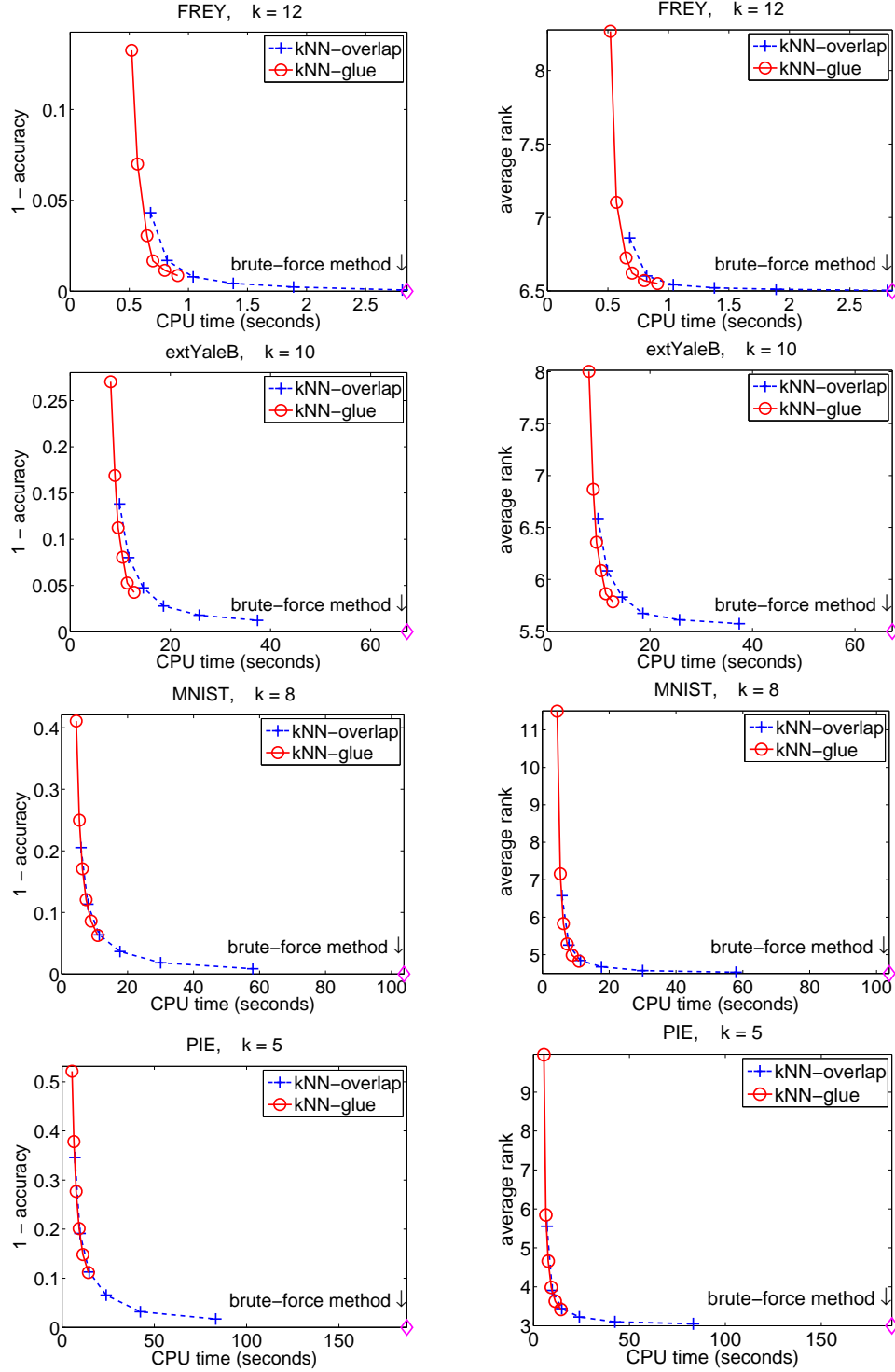
Figure 4: Graph quality versus running time for different data sets. Each row of the plots corresponds to one data set. The left column of plots shows the 1-accuracy measure. The right column shows the average-rank measure. Each plotted point corresponds to a choice of \alpha . From left to right on each curve, the \alpha values are 0.05, 0.10, 0.15, 0.20, 0.25, 0.30, respectively.
